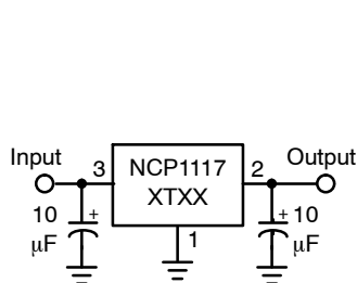
Figure 1. Fixed Output Regulator
